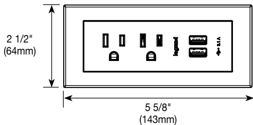
Basic Power Unit
