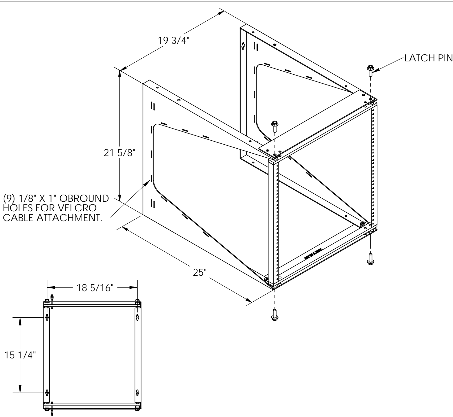
REAR VIEW
