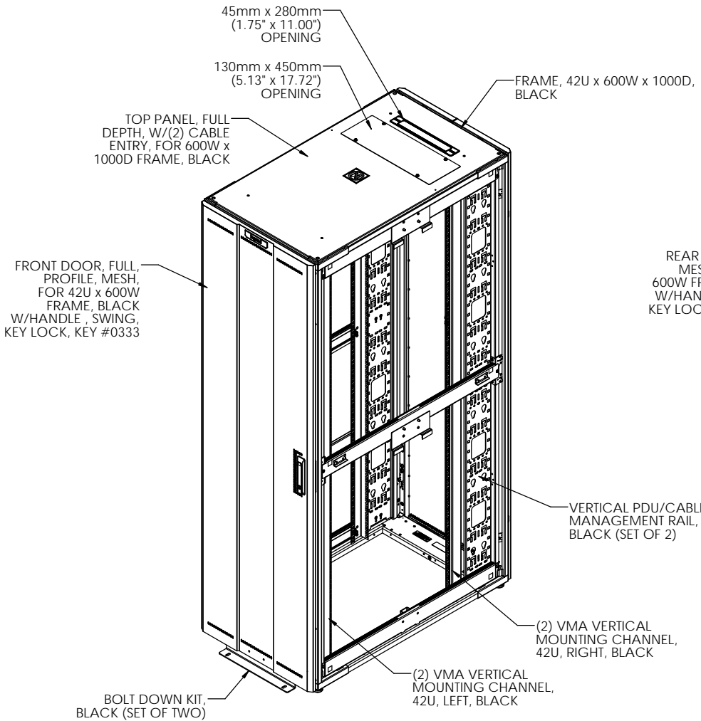
FRONT ISOMETRIC VIEW (SIDE PANELS REMOVED FOR VIEWING)
